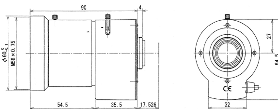
VT4Z1450MXJD / VT4Z1450MXJP
