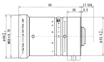
VT4Z1450MXJ
